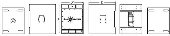
Dimension(W×H×D): 520×700×618mm
